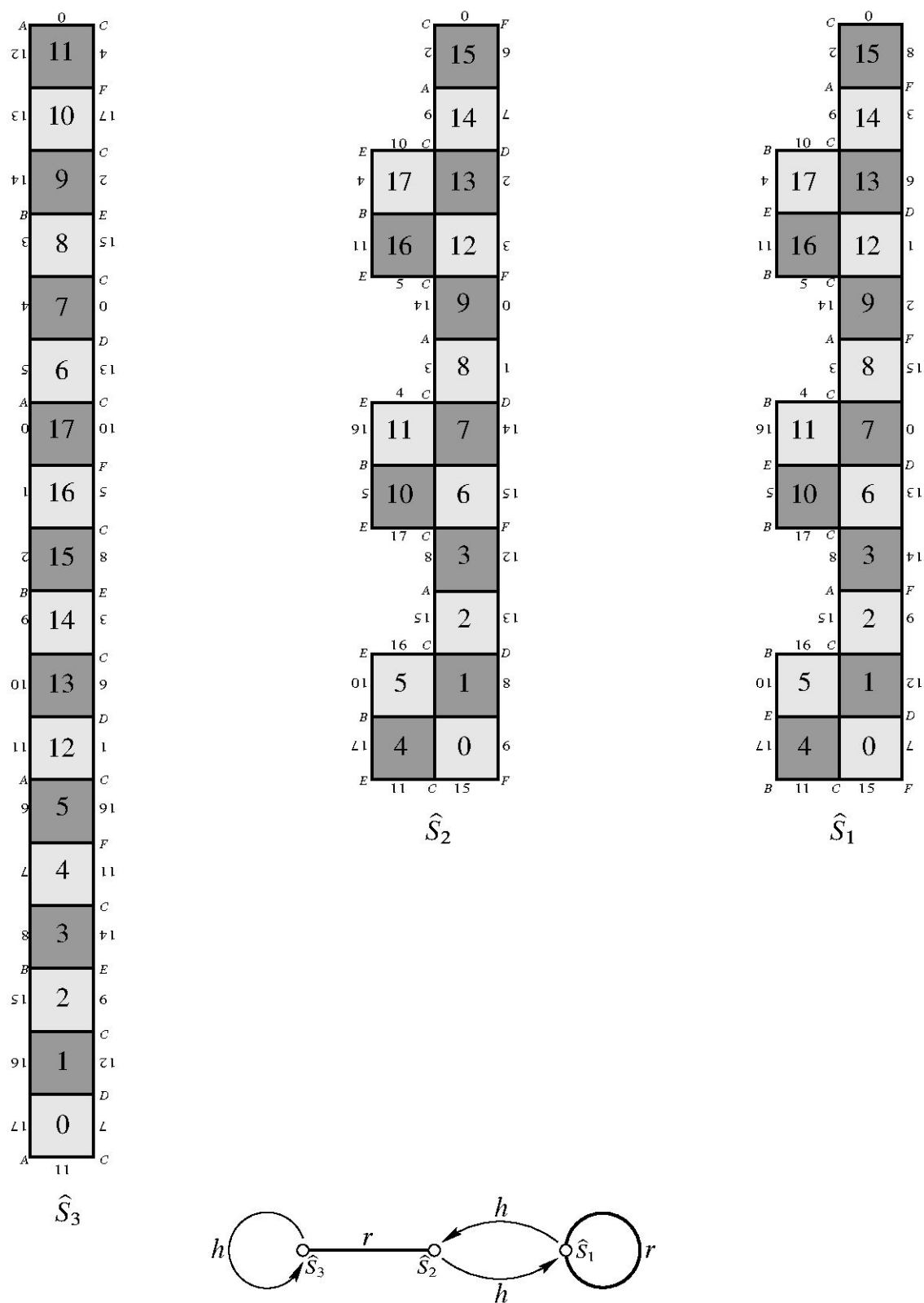
Figure 5. \mathrm{PSL}(2, \mathbb{Z}) -orbit of \hat{S} = \hat{S}_3 .
