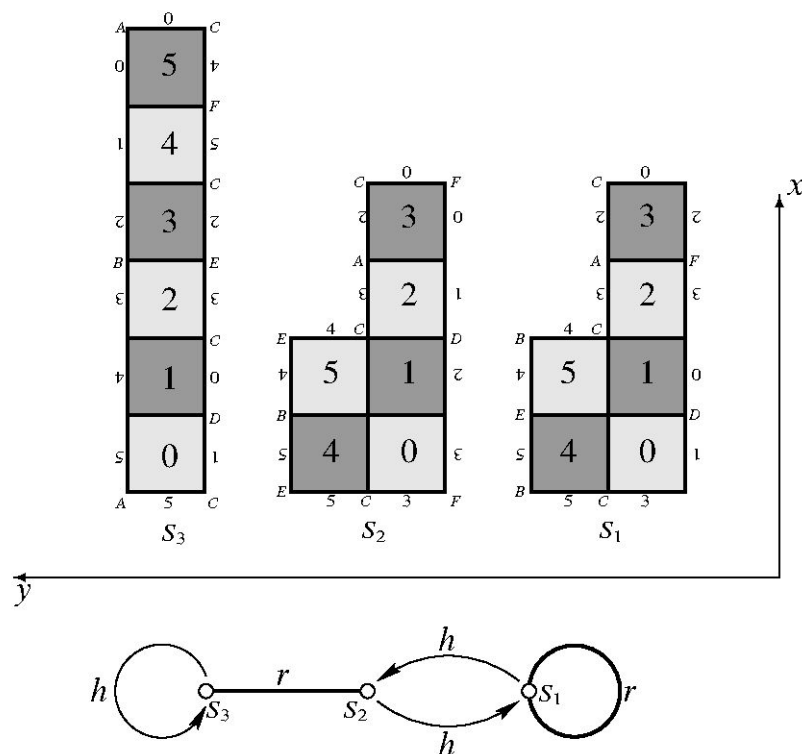
Figure 2. \mathrm{PSL}(2, \mathbb{Z}) -orbit of S .
