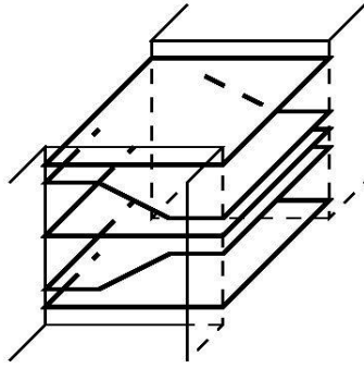
Figure 7. Foliation (\mathcal{F}_0^1|_{V_{j_*}}) .
