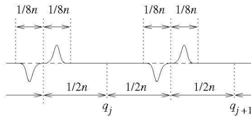
Figure 3. Function \chi_1 .
