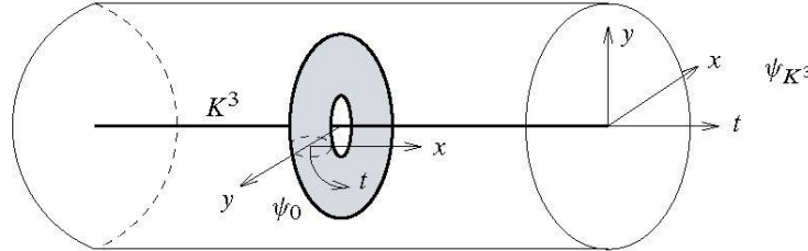
Figure 11. The 0-framed unknotted embedding \psi_0 .
