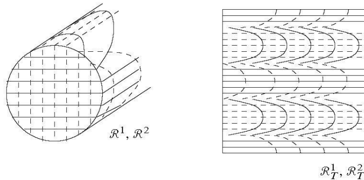
Figure 1. Foliations \mathcal{R}^1 , \mathcal{R}^2 , \mathcal{R}_T^1 , and \mathcal{R}_T^2 .
