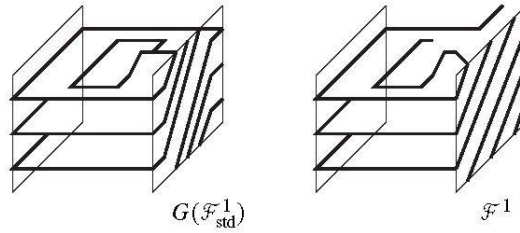
Figure 9. Proof of Lemma 3.13.
