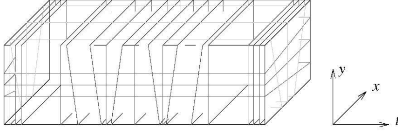
Figure 4. Total foliation (\mathcal{F}_{\text{std}}^i)_{i=1}^3 on [0, 1] \times [j/n, (j+1)/n]^2 .
