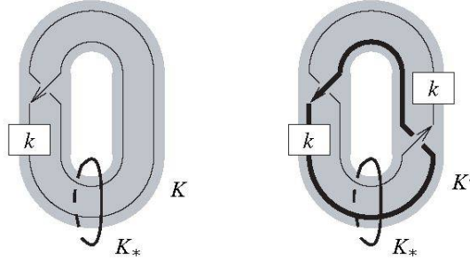
Figure 13. Double covering of a solid torus.
