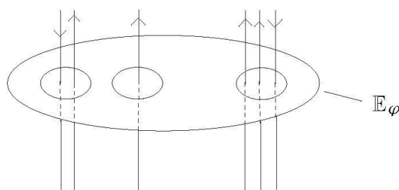
Figure 1.3. Properly embedded multi-disk.
