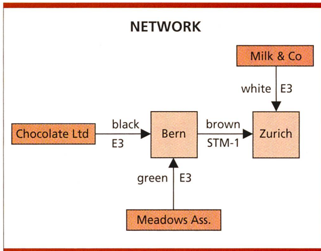
Fig. 5. Sample network.
