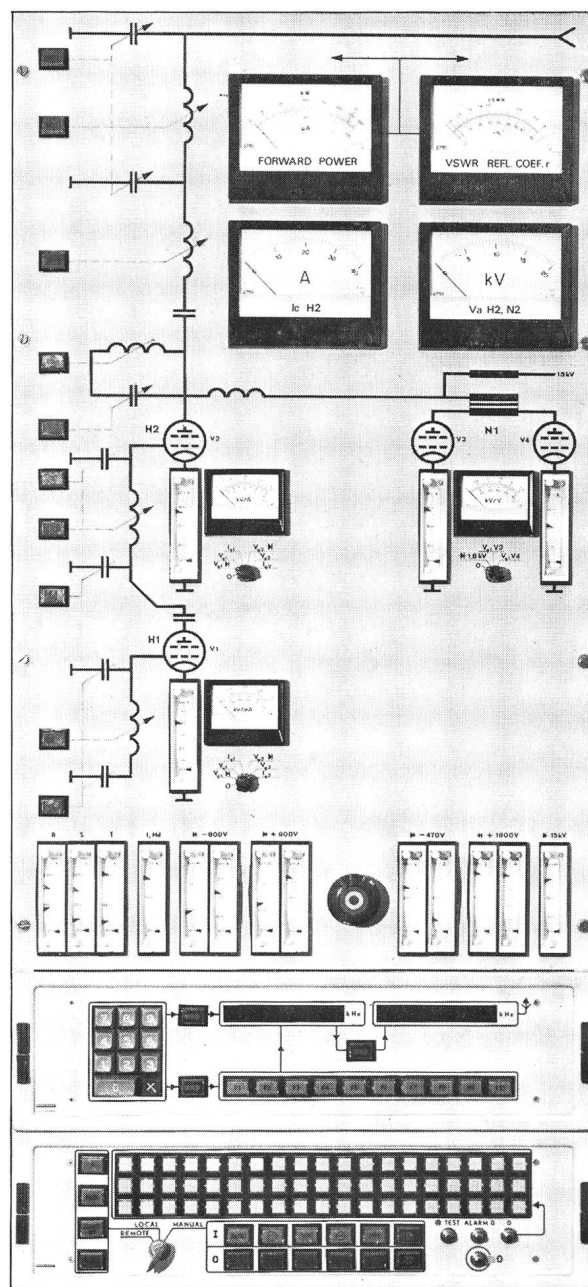
Control panel of the 250 kW automatic short-wave transmitter
