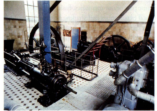
Uster 1980: Brewing vats at the Uster brewery with the last steam engine in the Zurich Oberland. Valve engine and cooling compressor from 1897
