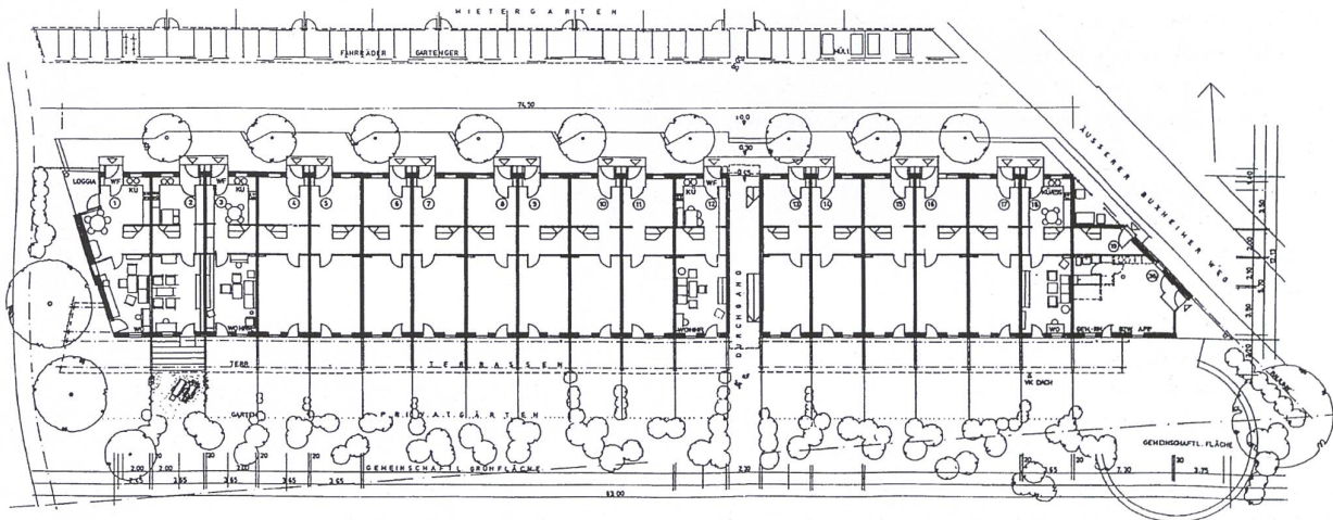
Grundriß Erdgeschoß
