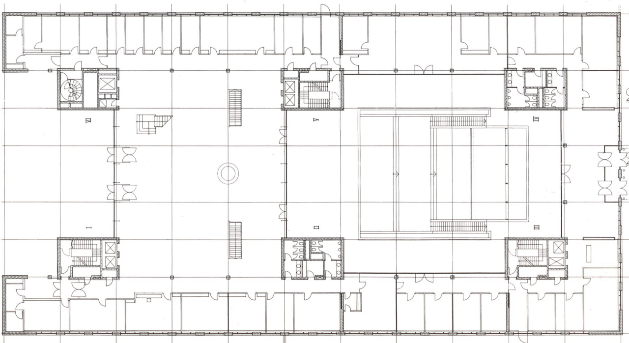
Grundriß Erdgeschoß
