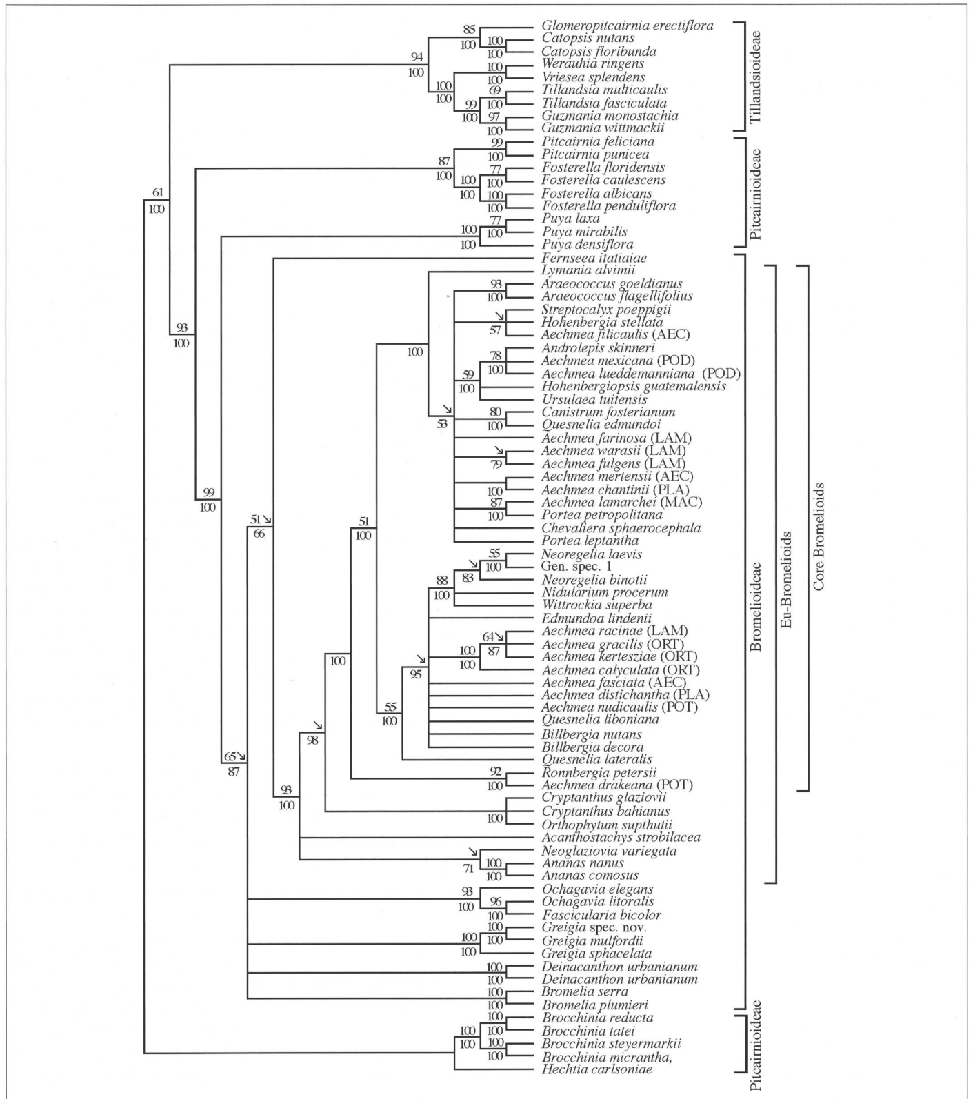
Fig. 1. – 50% Majority rule consensus tree of 49400 trees obtained from four runs of Bayesian analysis of the combined dataset implementing the GTR+G+I model. Posterior probabilities are given above branches. (Abbreviations: Aechmea subgenera, AEC: Aechmea; POD: Podaechmea; PLA: Platyaechmea; LAM: Lamprococcus; ORT: Ortgiesia; POT: Pothuava; MAC: Macrochordion).
