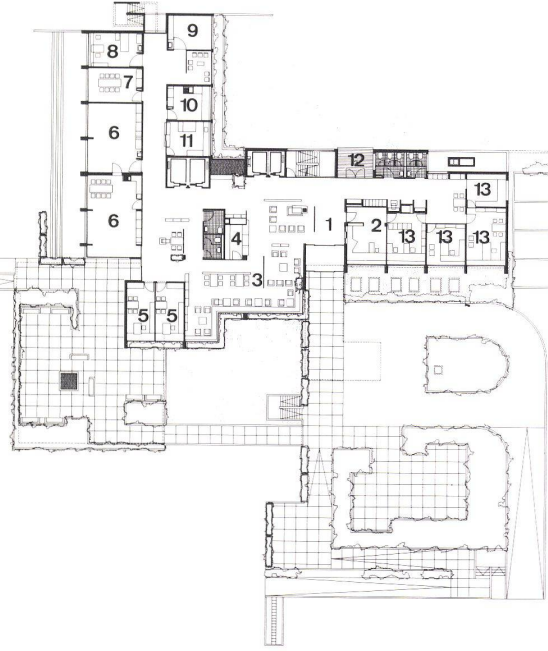
4 Grundriß eines Pflegegeschosses 1:700. Plan of a hospitalization floor.
