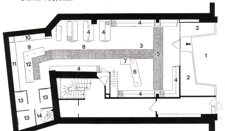
Grundriß / Plan 1:200
