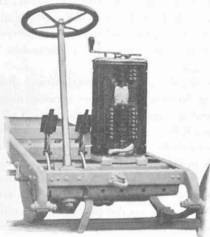
Fig. 3. — Controller.
