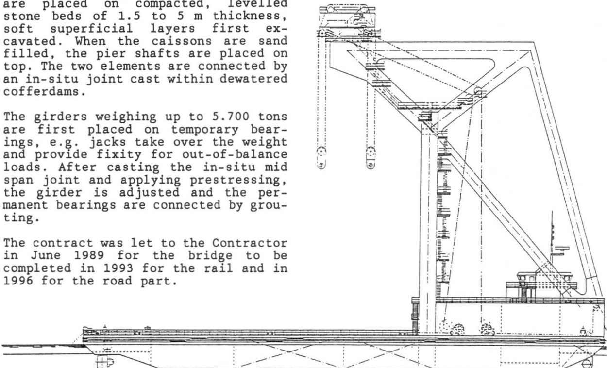
Fig. 3.5 The catamaran crane vessel.
