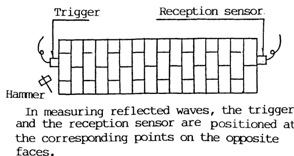
Fig. 6 Nondestructive Test
