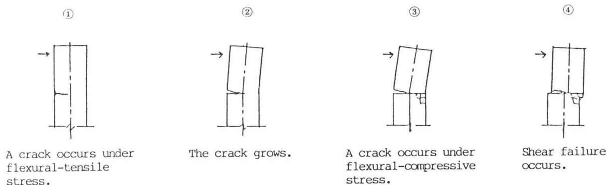
Fig.10 Failure Process [5]
