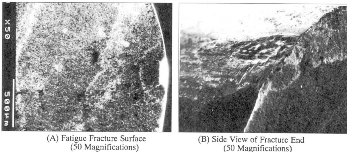
Fig. 4 An Example of Fatigue Failure of Prestressing Wire
