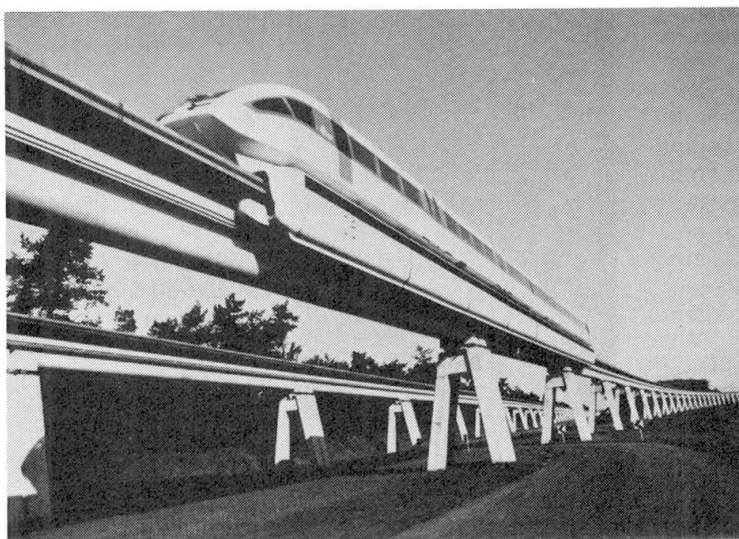
Fig. 1 Concrete guideway for the TRANSPRAPH Test Facility Emsland, 1st construction phase with MagLev vehicle
