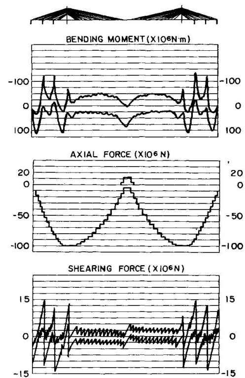
Fig. 4 Section forces
