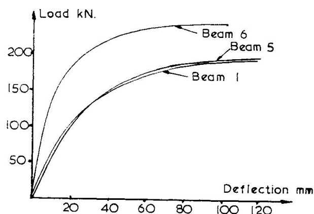
Fig. 6 Load deflection curves
