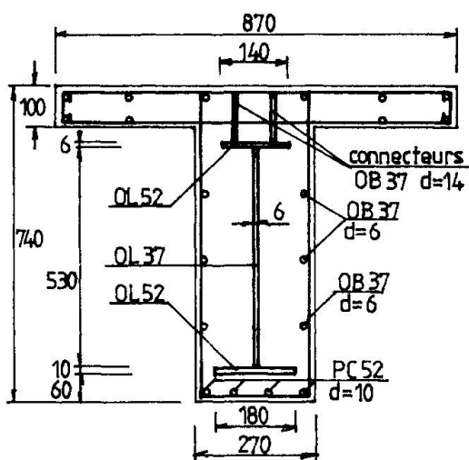
Fig.2 Section transversale [mm]
