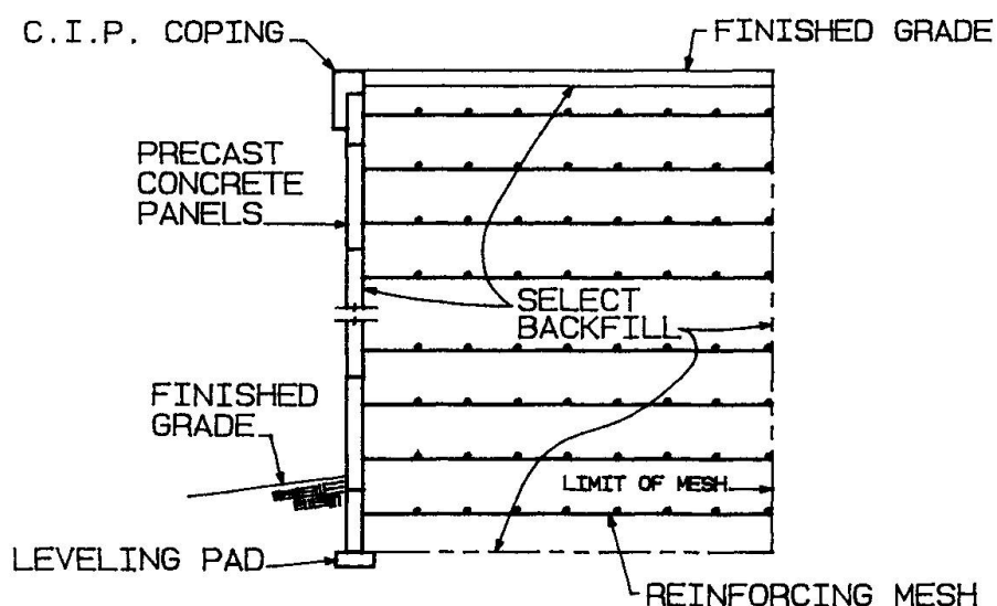
FIGURE 1. TYPICAL SECTION THROUGH R.E. WALL
