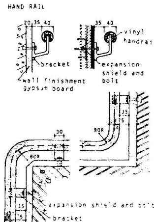
Fig. 2d Handrail
