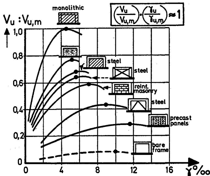
Fig. 42b: Several infill materials and techniques lead to different strength and ductilities (SUGANO, 1981)
