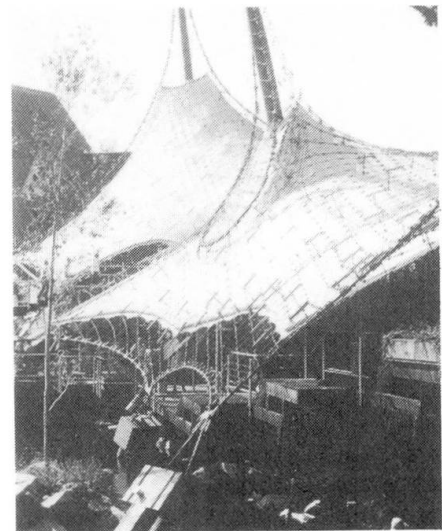
Fig 26 West German Pavilion - Expo 67
