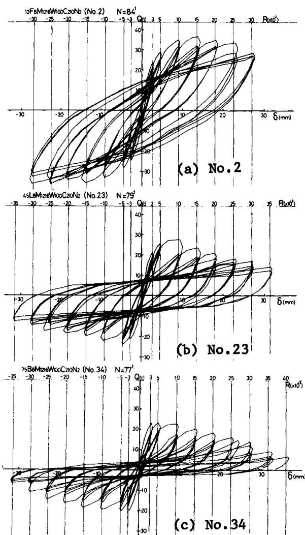
Fig. 11 Shear-Deflection Relationship
