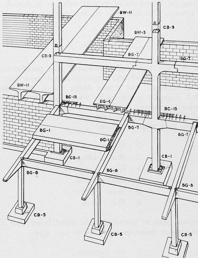
Fig. 8 - Typical Connections.
