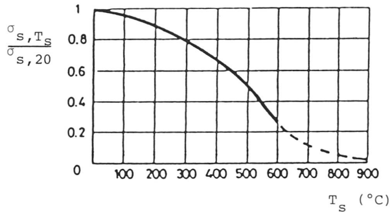
Figure 14 : Quotient between effective yield stress \sigma_{S, T_S} at elevated temperature T_S and yield stress at room temperature \sigma_{S, 20} as a function of steel temperature T_S . The curve applies to steel grades Fe 360 to Fe 510 with an accuracy, which is sufficient for practical purposes (11)
