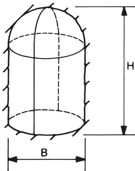
Fig. 3 Large underground chamber with statically favourable shape
