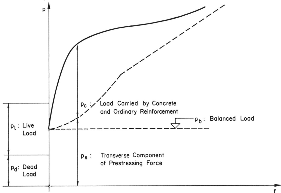
Fig. 10. Schematic Load - Deflection Curve of a Prestressed Flat Slab
