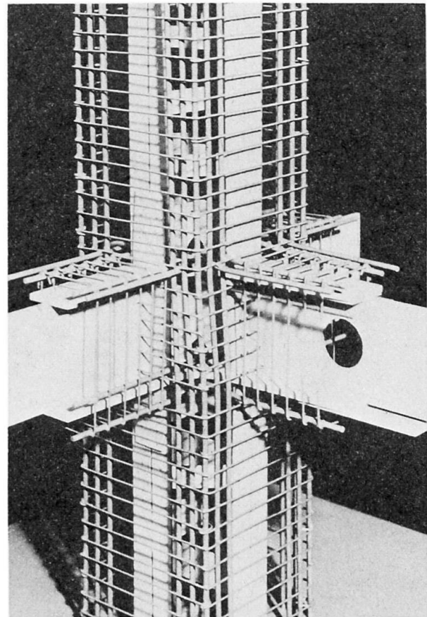
Fig. 20 Connection in building for mixed construction (model).
