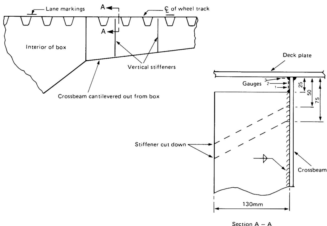
Fig.5 Crossbeam stiffener
