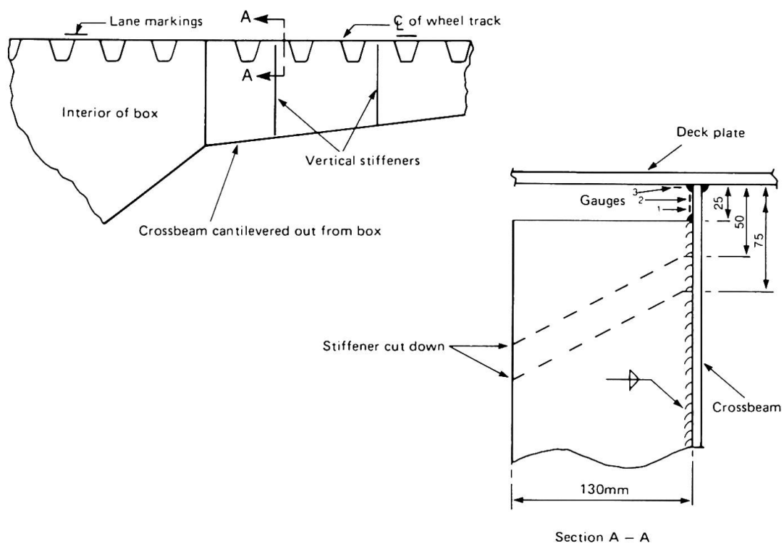
Fig.5 Crossbeam stiffener
