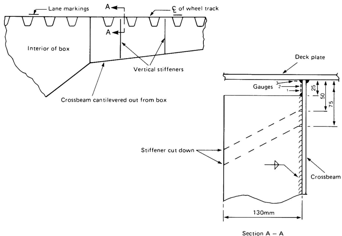
Fig.5 Crossbeam stiffener
