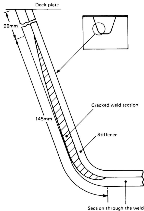
Fig.2 Crack location in trough to crossbeam weld
