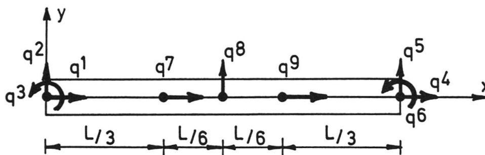
Fig. 10 Beam element with 9 degrees of freedom
