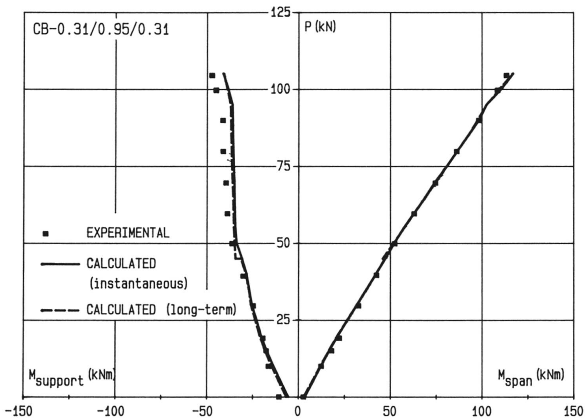
Fig. 7 Evolution of bending moments for beam CB-0.31/0.95/0.31
