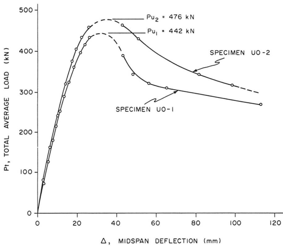
Fig.5 Load-deflection curves
