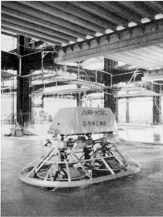
Photo 6 Surf robot
