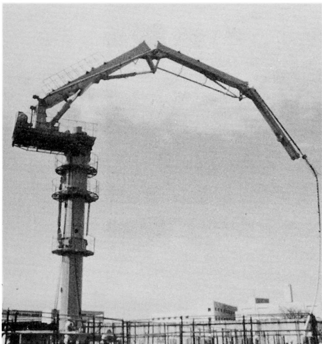
Photo 4 Con-disk crane
