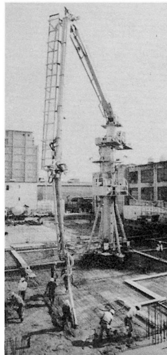
Photo 5 Placing crane
