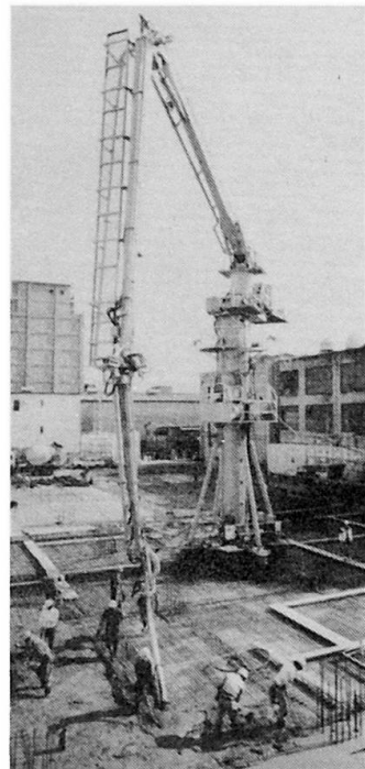
Photo 5 Placing crane
