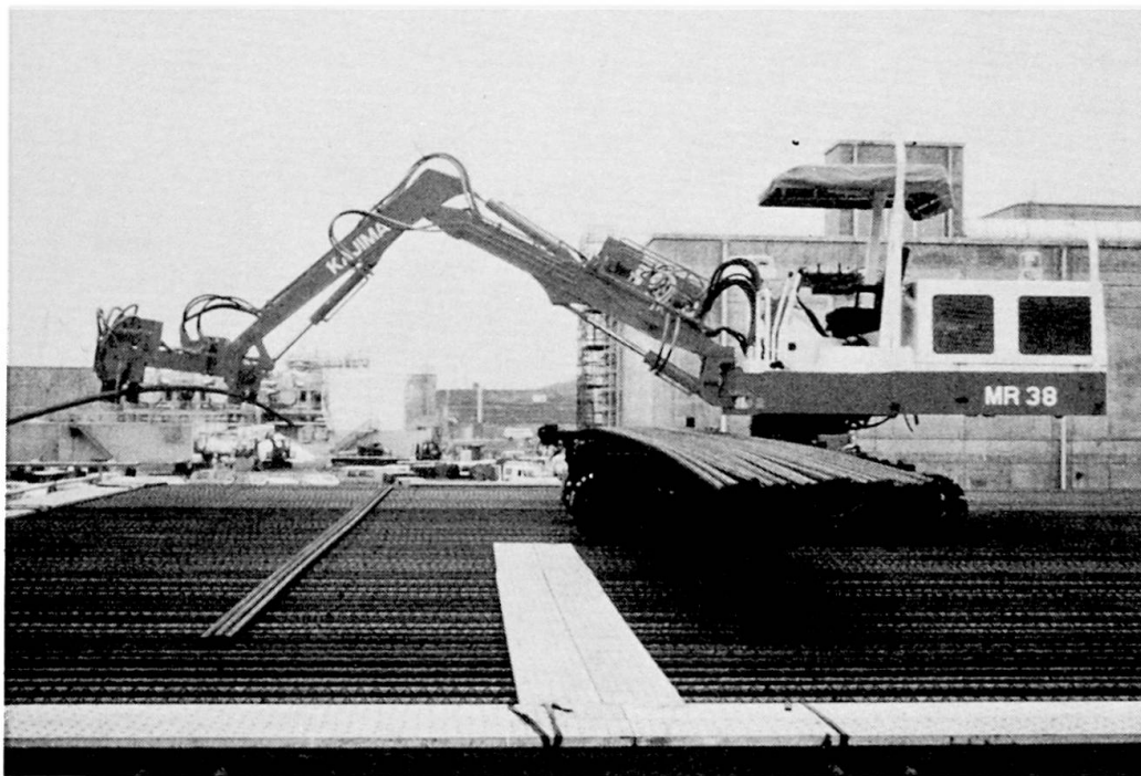
Photo 1 Heavy bar assembling robot
