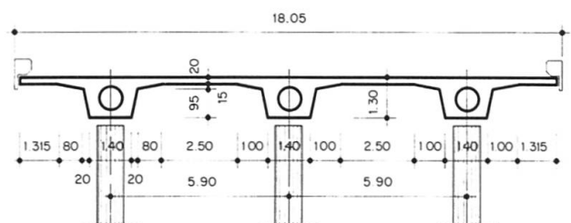
Fig. 1 Cross-section of the wadi crossing
