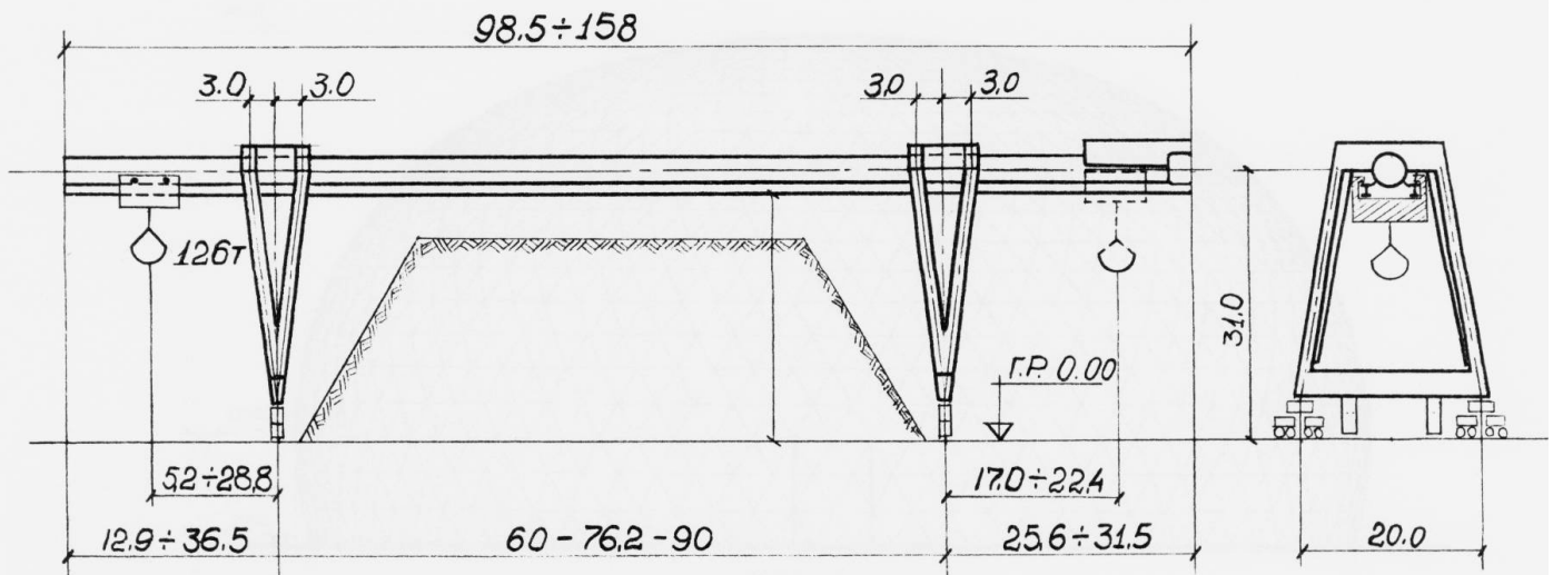
Fig. 1 A Loading Crane of a Pipe-girder Type
