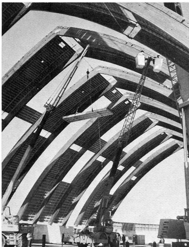
Fig. 3 Stressed skin panels lifted into place
