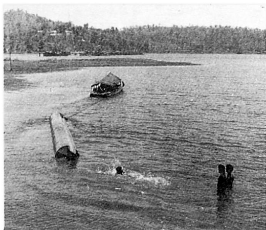
Photo.3 1000mm diameter casing being towed to site
