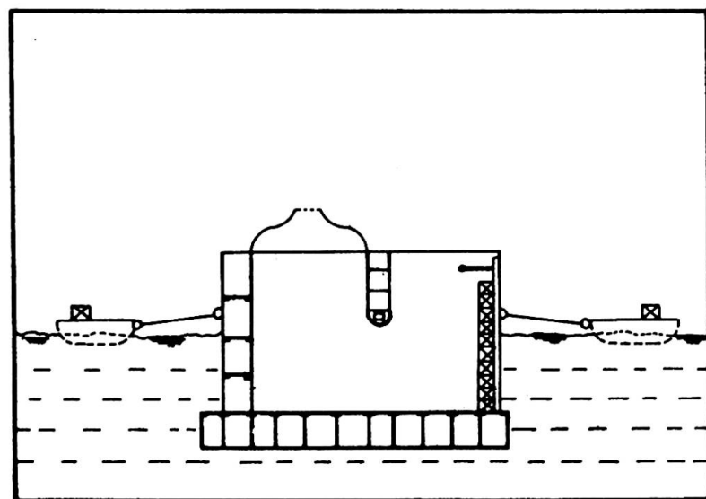
Fig. 3.c Towing
