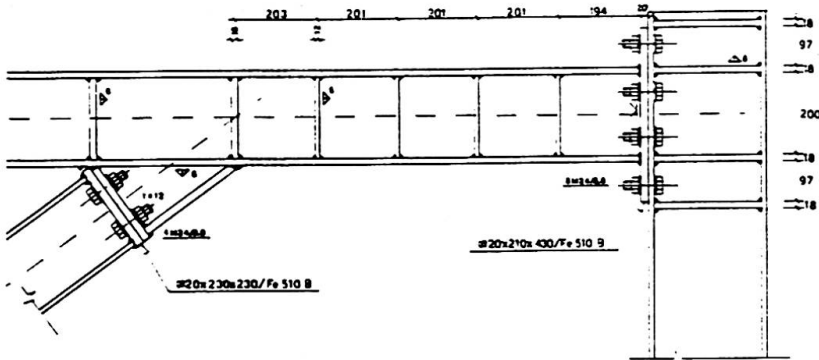
Fig. 1 Details of the active links
