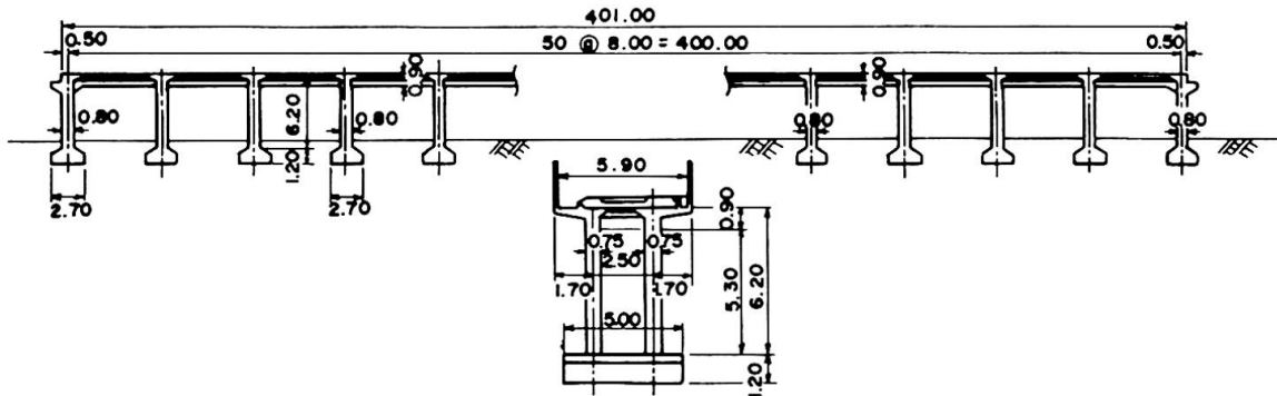
Fig. 1 General View
