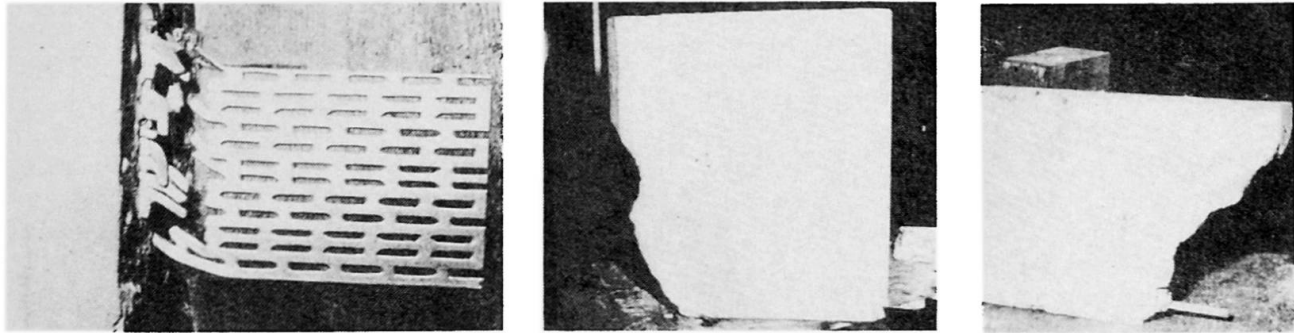
Fig. 16.1&2 Final failure in shear for no. 1&2 Fig. 16.3 Final failure by cracking of concrete for no. 3 Fig. 16.4 Final failure by cracking of concrete for no. 4
