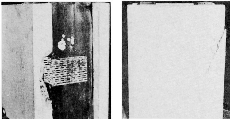
Fig. 16.5 Final failure by cracking of concrete edge for no. 5 Fig. 16.6 Final failure in shear/cracking of concrete, no. 6
