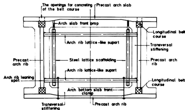
Fig. 5 - Cross section of the arches' assembly portion
