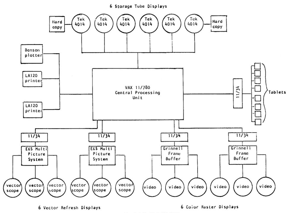
SCHMATIC EQUIPMENT CONFIGURATION Figure 1
