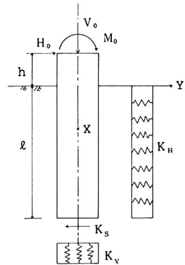
Fig. 6 Structural model
