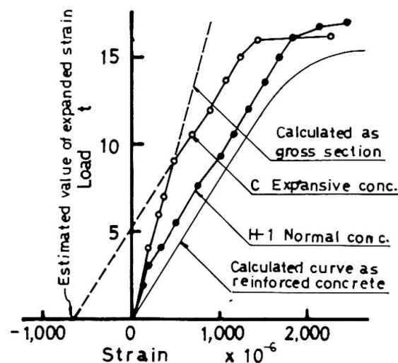
Fig. 4 Load-strain diagram
