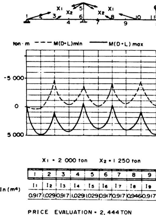
Fig. 11. Optimum Design
