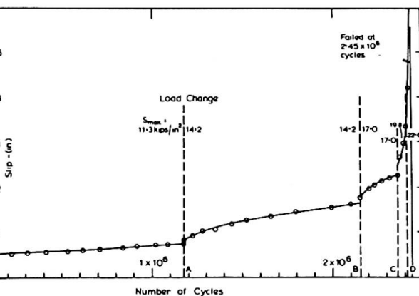
FIG 6 PUSH-OUT SPECIMEN PR5 - HISTORY OF SLIP
