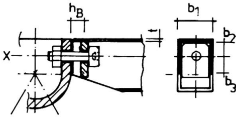
Fig. 2 Mero-Plus connector
