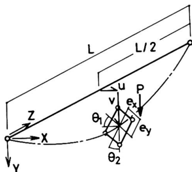
Fig. 7 Lattice beam under eccentric load
