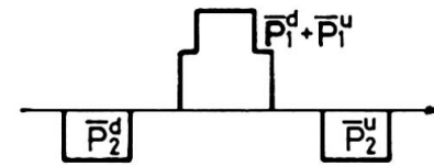
Fig.10 Double track load(i)
